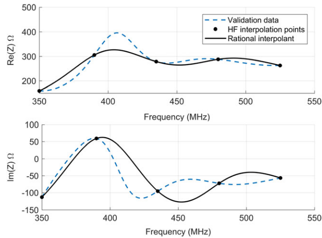
FIGURE 5 Barycentric rational interpolation of the input impedance as a function of frequency using only the high-fidelity (HF) data with n + 1 = 5
