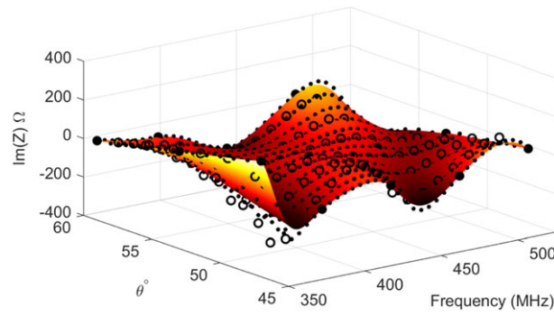
FIGURE 9 Blended rational interpolation of the imaginary part of the input impedance using the high-fidelity (HF) and low-fidelity (LF) two-dimensional data. HF data are indicated by large dots, LF data by small dots, validation data by open circles, and the resulting rational interpolant by the surface
