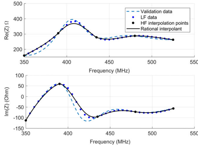
FIGURE 8 Blended rational interpolation of the input impedance as a function of frequency using the (high-fidelity) HF and (low-fidelity) LF data with n + 1 = 5 and m + 1 = 36
