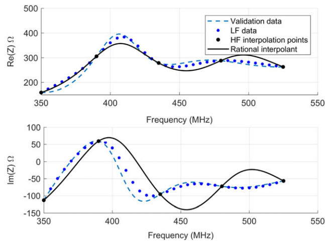
FIGURE 6 Barycentric rational interpolation of the input impedance as a function of frequency using the high-fidelity (HF) and low-fidelity (LF) data with n + 1 = 5 and m + 1 = 36
