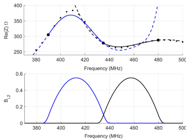
FIGURE 7 Local models p_i (top panel) and blending functions B_{i,2} (bottom panel) used in the blended rational interpolation scheme. Small dots indicate the LF data and large dots the HF data—both sets taken from the middle 2 intervals of the top panel of Figure 6. The blue curves represent the functions relating to the interval between the first 2 HF data points, and black curves those relating to the interval between the last 2 HF data points. Solid lines indicate the local models on their relevant domains, while dashed lines indicate the extensions of the local models outside the relevant intervals
