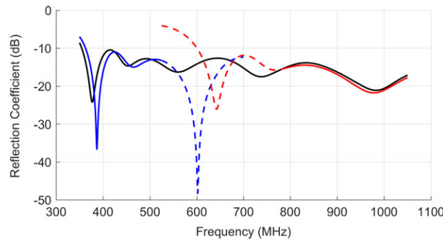
FIGURE 3 Comparison between the (high-fidelity) HF and (low-fidelity) LF model reflection coefficients. The blue line is the low band LF model, the red line the high band LF model, and the black line the HF model. Dashed lines indicate ignored edge effect regions in the coarse model frequency bands
