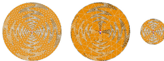
FIGURE 4 Comparison of the simulation meshes of the high-fidelity model (left), the low band low-fidelity (LF) model (centre) and the high band LF model (right)
