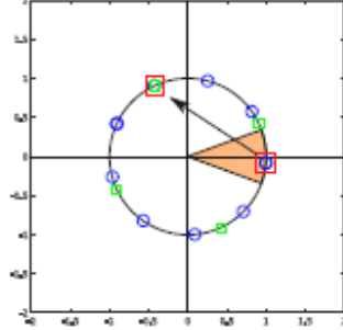
Figure 4: Intersection of U_i (blue circles, u = 9 ) and S_i (green squares, s = 4 ), relocating the aliased {}_u\lambda_i (red square).
