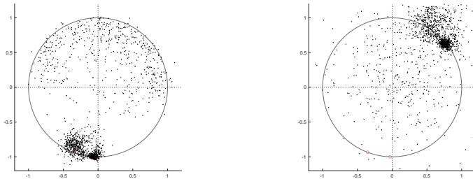
Figure 7: Joint {}^7\lambda_{1,2} (at the left) and {}^9\lambda_{1,2} (at the right) of (14) for all noise realizations.
