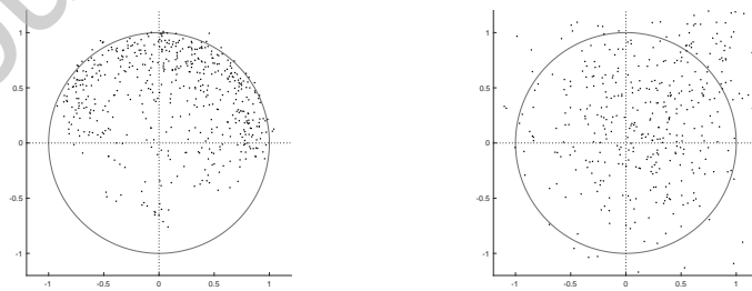
Figure 10: Candidate cluster for (14) retrieved in {}^uL (left) without associated cluster in {}^sL (right).
